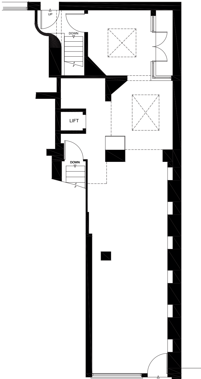
GROUND FLOOR
