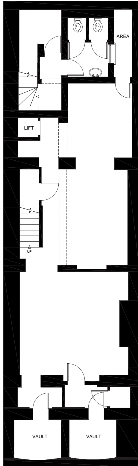
BASEMENT
