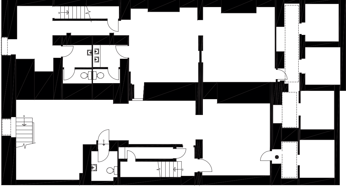
BASEMENT
